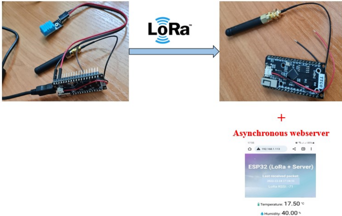
Fig. 1 Sensor node architecture
