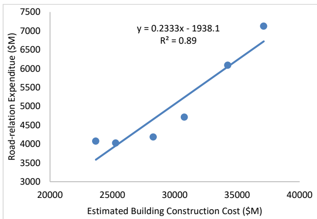
Fig. 3 Road-related expenditure vs. estimated cost of building construction
