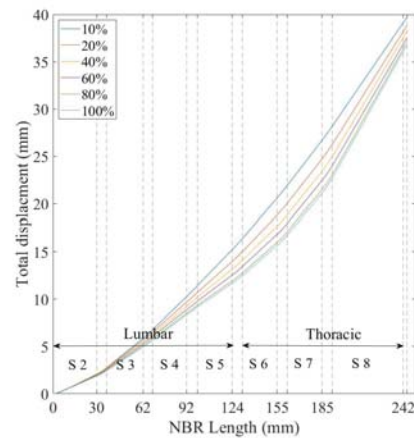
Fig. 11 Stress and Displacement of NRB cord
