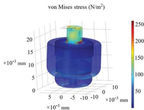
Fig. 5 Connector stress
