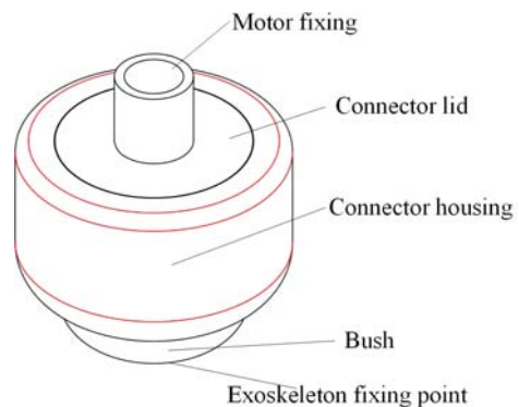
Fig. 3 Connector
