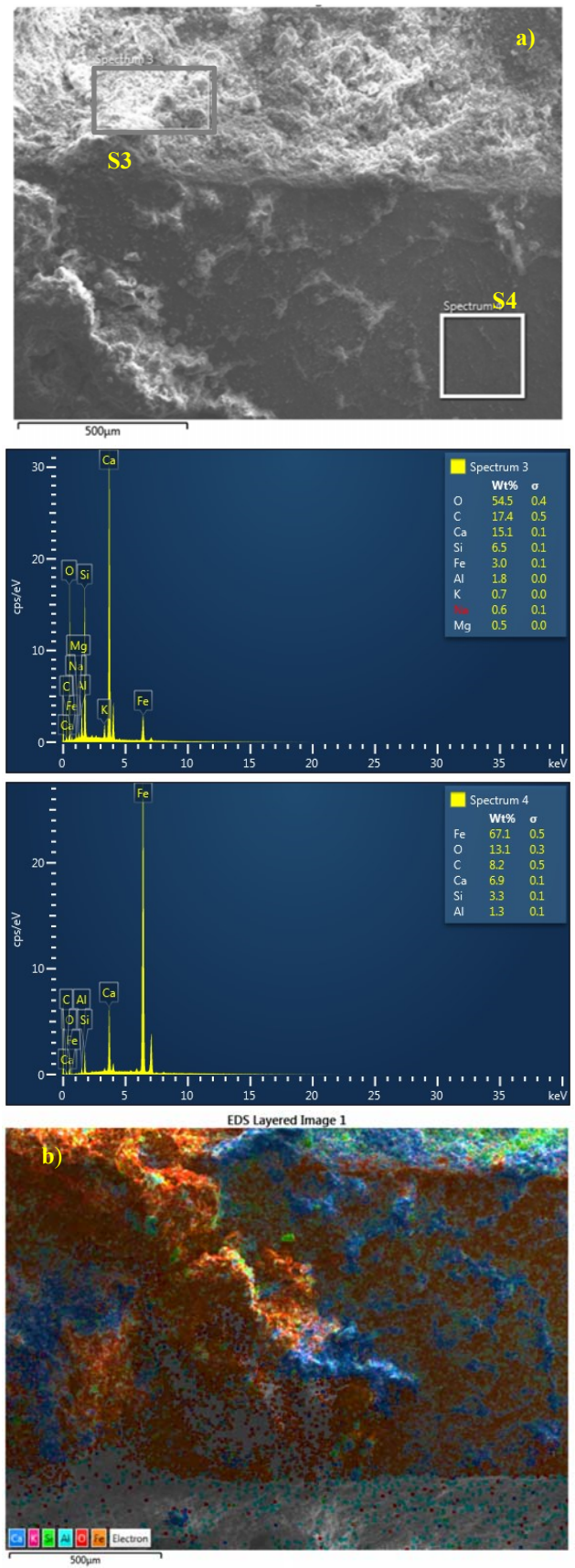
Fig. 6 SEM-EDX analysis of the S15 sample
