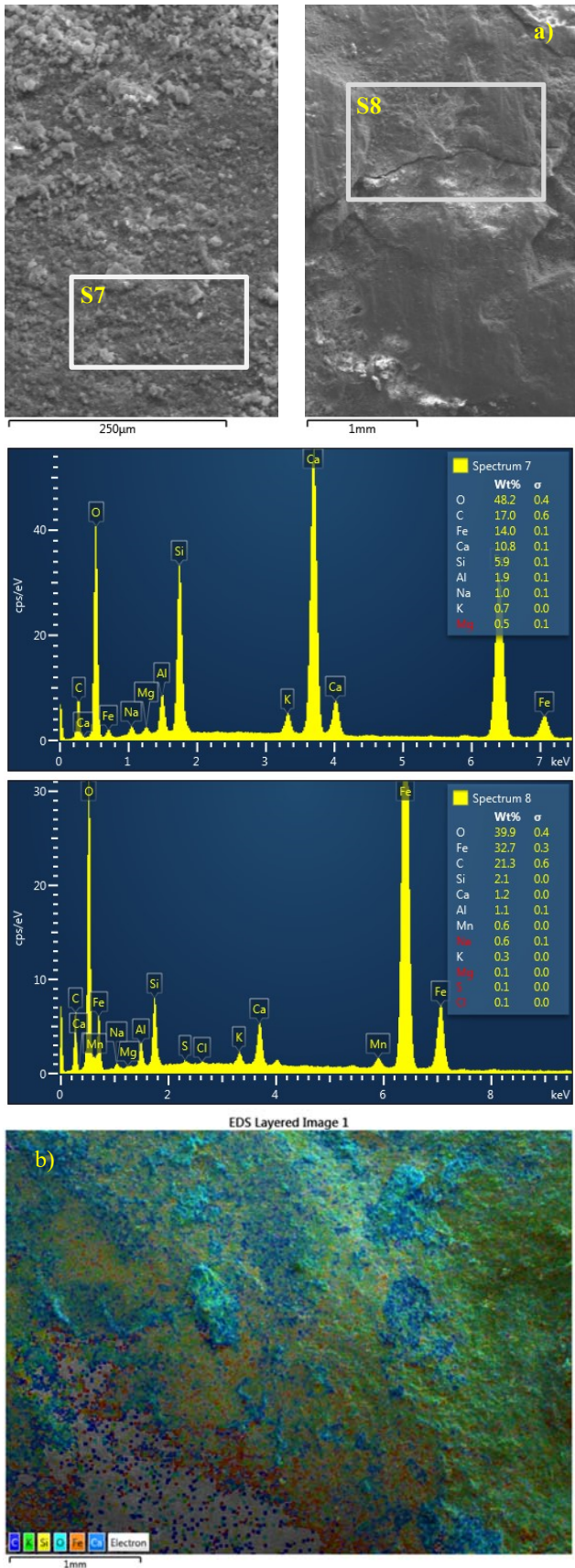
Fig. 5 SEM-EDX analysis of the S0 sample
