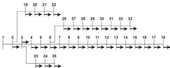
Fig. 1 Structure of the IEEE 33 Node Network [17]
