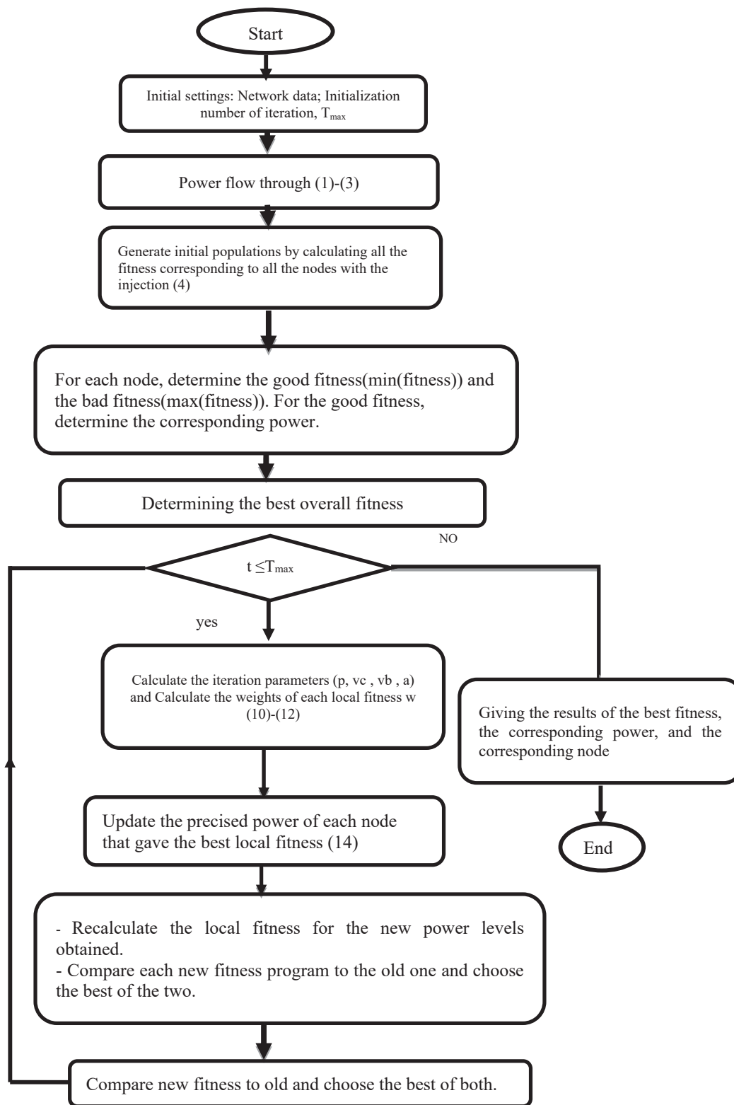
Fig. 3 Flowchart of the Method by the SMOA
