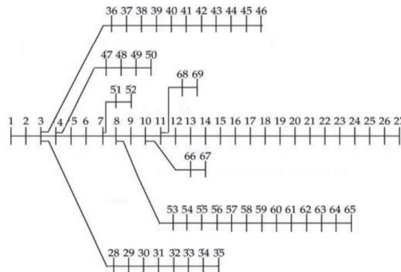
Fig. 2 Structure of the IEEE 69 Nodes Network [18]
