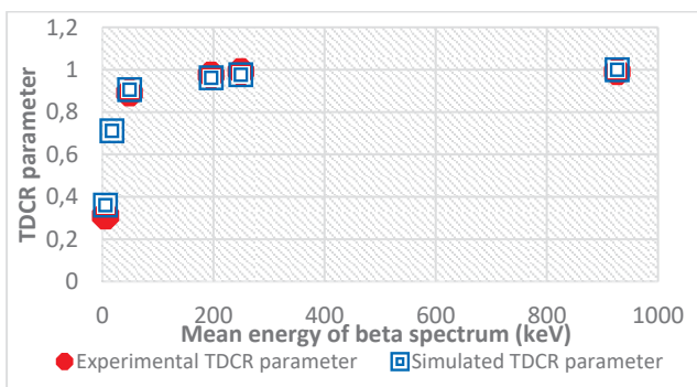
Fig. 4 Experimental and simulated TDCR detection efficiency
