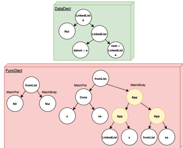
Fig. 7 LinkedList AST
