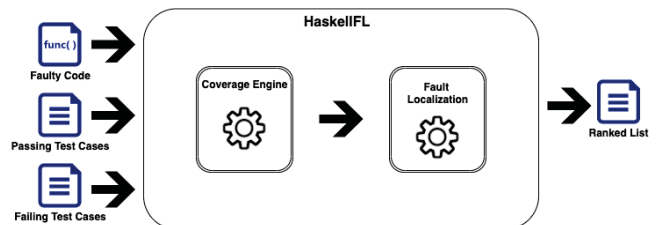
Fig. 5 HaskellFL architecture
