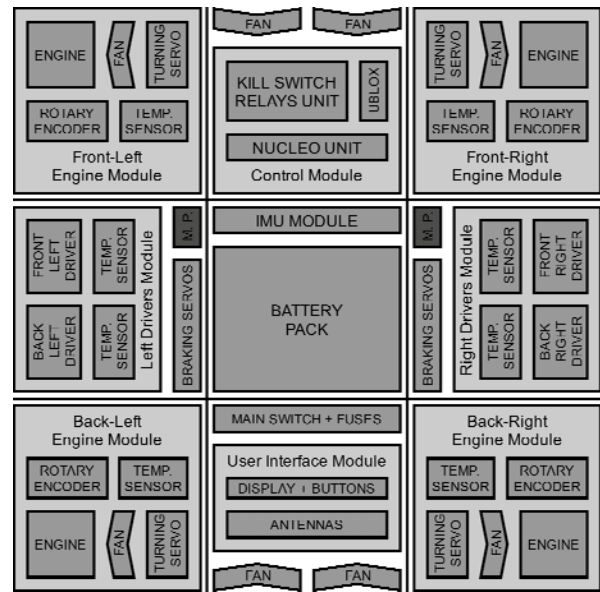
Fig. 3 Physical schematics of the ARP
