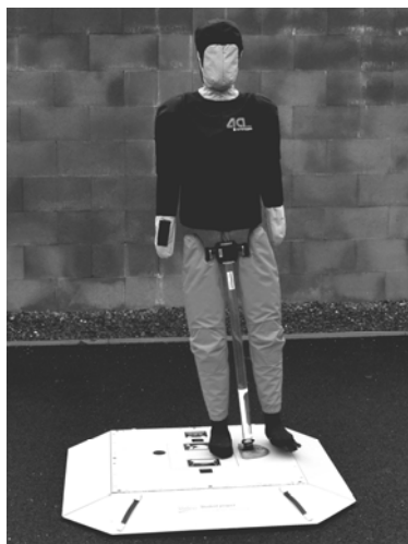
Fig. 6 Prototype with the mounted pedestrian
