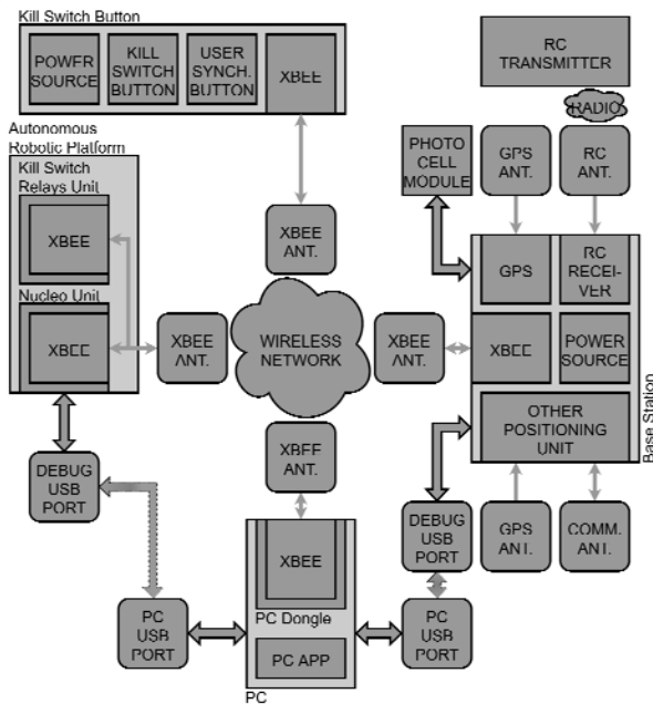
Fig. 2 Block schematics of the whole system
