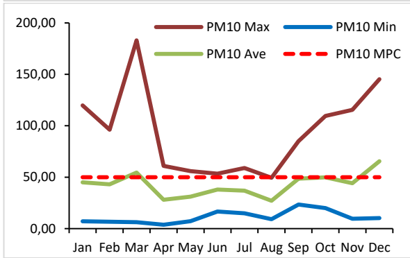
Fig. 2 Maximum, minimum and average monthly concentrations of PM 2.5 and PM 10 in 2020
