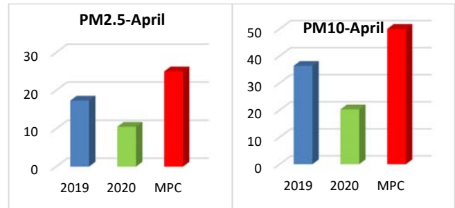
Fig. 4 Average monthly concentrations of PM 2.5 and PM 10 in April of 2019 and 2020
