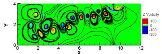
Fig. 5 Streamline pattern in the wake of a swimming nematode superimposed on z-vorticity field at Re = 1200
