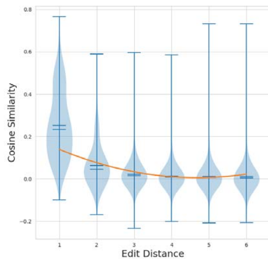
(a) Correlation between Edit distance of k-mers and cosine similarity of k-mers embeddings
