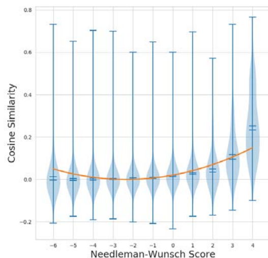
(b) Correlation between Needleman-Wunsch score of k-mers and cosine similarity of k-mers embeddings
