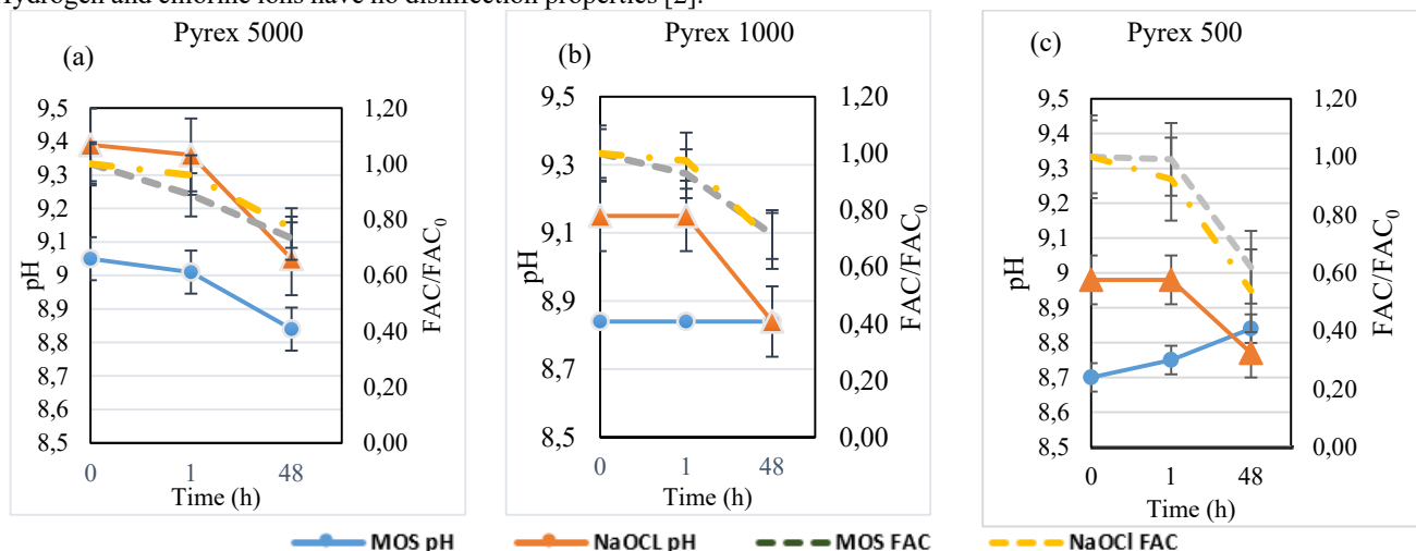
Fig. 1 Variation of pH and FAC over time for MOS & HYPO solutions in Pyrex containers (a) 5000 ppm, (b) 1000 ppm, (c) 500 ppm, (solid line for pH, dotted line for FAC)
