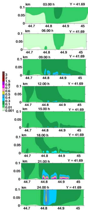
Fig. 5 (a) Dust concentration (MAC) distribution within 24 hours in the surface layer of the atmosphere in three vertical planes located along a parallel ( Y = 41.69^\circ )
