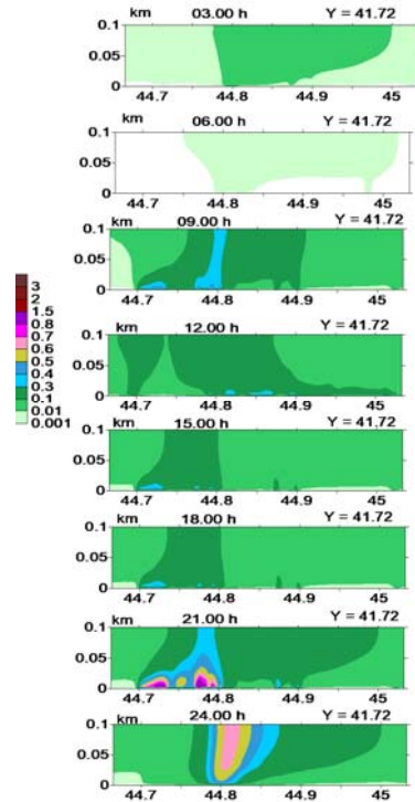
Fig. 5 (b) Dust concentration (MAC) distribution within 24 hours in the surface layer of the atmosphere in three vertical planes located along a parallel ( Y = 41.72^\circ )
