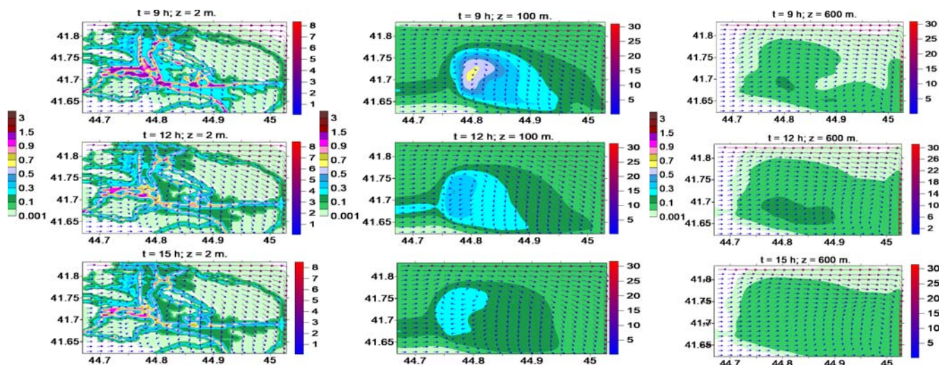
Fig. 3 Wind velocity (m/sec) and dust concentration (MAC) distribution, when t = 9, 12, and 15 h, at 2, 100, and 600 m height above the earth surface
