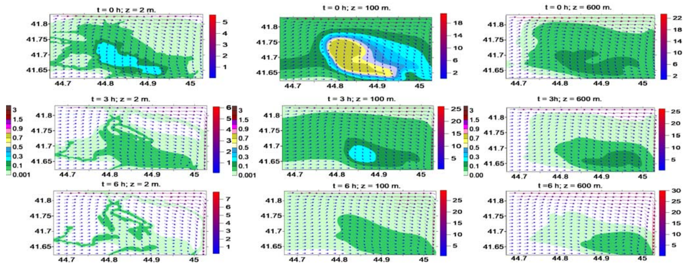
Fig. 2 Wind velocity (m/sec) and dust concentration (MAC) distribution, when t = 0, 3, and 6 h, at 2, 100, and 600 m height above the earth surface
