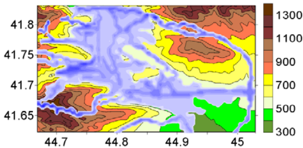
Fig. 1 Tbilisi terrain heights (m) and distribution of pollution sources. Accurate geographic coordinates are marked off the axes
