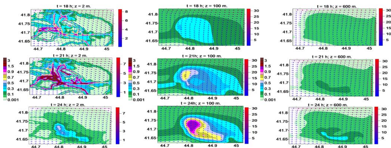
Fig. 4 Wind velocity (m/sec) and dust concentration (MAC) distribution, when t = 18, 21, and 24 h, at 2, 100, and 600 m height above the earth surface
