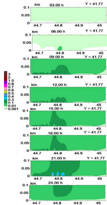
Fig. 5 (c) Dust concentration (MAC) distribution within 24 hours in the surface layer of the atmosphere in three vertical planes located along a parallel ( Y = 41.77^\circ )
