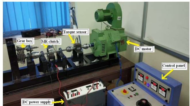
Fig. 3 Experimental test rig for testing the MR Clutch
