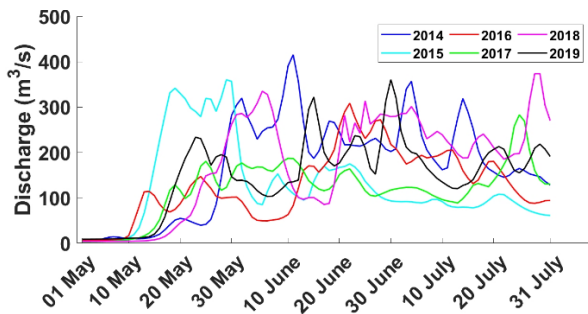
Fig. 2 Annual Sagavanirktok River discharge (m 3 /s) from USGS PUMP STA 3
