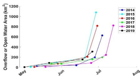
Fig. 7 Estimated discharge overflow and open water area (km 2 ) for the Sagavanirktok River delta
