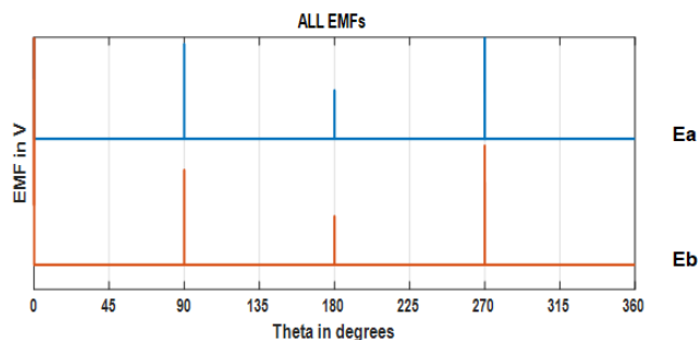
Fig. 20 Fully-pitched 4/2 SRG maximum output EMF E_a and E_b waveforms at stator and rotor teeth angles ( 90^\circ, 90^\circ )
