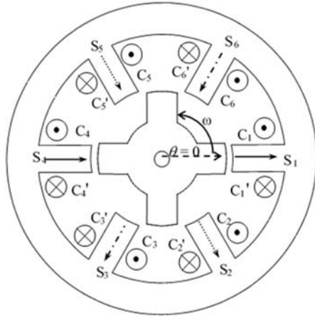
Fig. 7 Short-pitched 6/4 SRG ( p = 1 ) [10]
