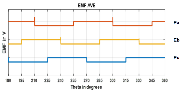
Fig. 13 Short-pitched 6/4 SRG output EMF Ea, Eb and Ec waveforms at stator and rotor teeth angles (45°, 45°)
