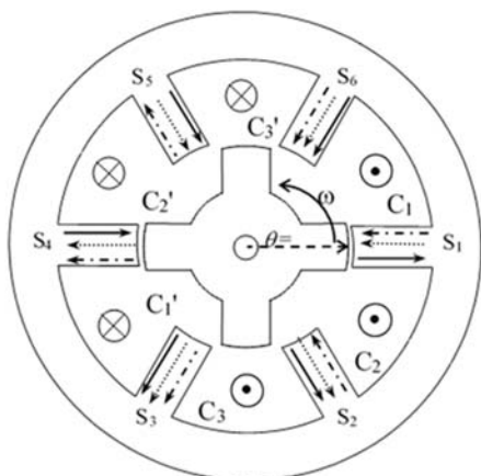
Fig. 17 Fully-pitched 6/4 SRG ( \rho = 3 ) [10]
