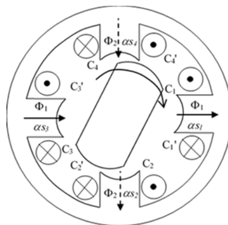
Fig. 6 Short-pitched 4/2 SRG ( \rho = 1 ) [10]
