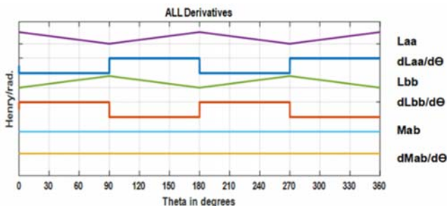
Fig. 9 Short-pitched 4/2 SRG self-inductances, its derivatives and zero- mutual inductances waveforms at stator and rotor teeth angles (90°, 90°)
