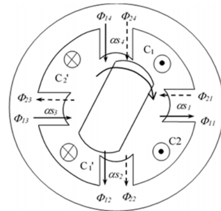
Fig. 16 Fully-pitched 4/2 SRG ( \rho = 2 ) [10]
