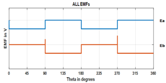
Fig. 10 Short-pitched 4/2 SRG maximum output EMF E_a and E_b waveforms at stator and rotor teeth angles (90°, 90°)
