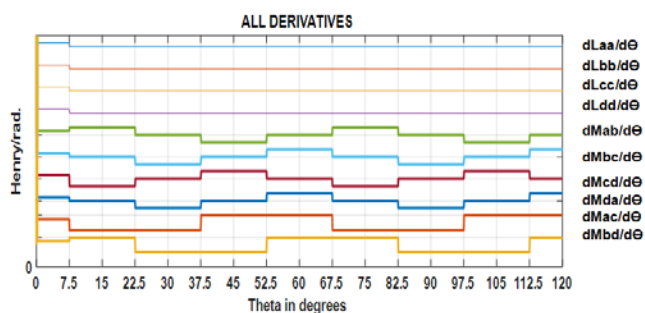
Fig. 25 Fully-pitched 8/6 SRG all derivatives waveforms at stator/rotor tooth angles (15°, 30°)
