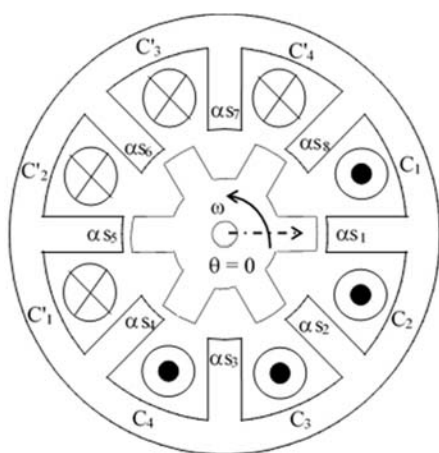
Fig. 18 Fully-pitched 8/6 SRG ( \rho = 4 ) [10]
