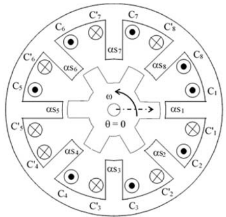
Fig. 8 Short-pitched 8/6 SRG ( p = 1 ) [10]
