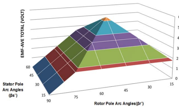
Fig. 14 The output total EMF per unit current versus \beta_s and \beta_r for 6/4 short-pitched SRG: Unipolar, 2-phase excitation
