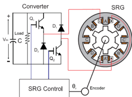
Fig. 1 Drive system of SRG [5]
