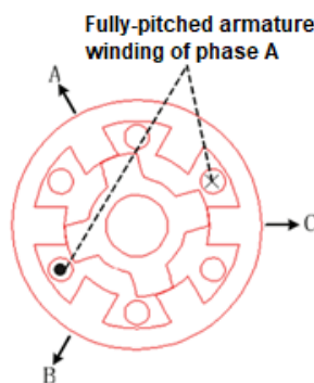
Fig. 4 Fully-pitched doubly salient configuration [9]
