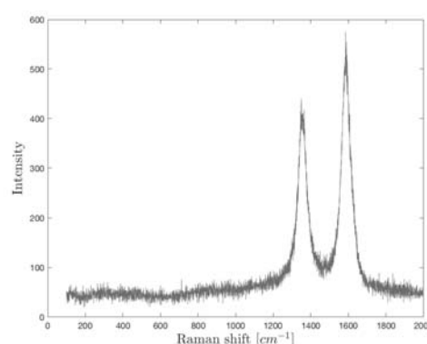
Fig. 6 The experimental outcome for the first sensor based on GO under vacuum chamber
