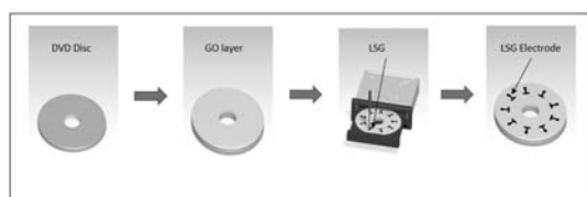
Fig. 1 The overall process of patterning LSG electrodes
