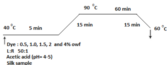
Fig. 1 Dyeing process
