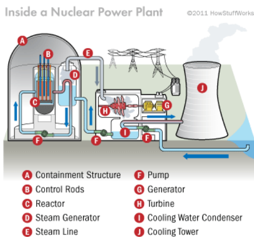
Fig. 3 Nuclear reactor overview [15]
