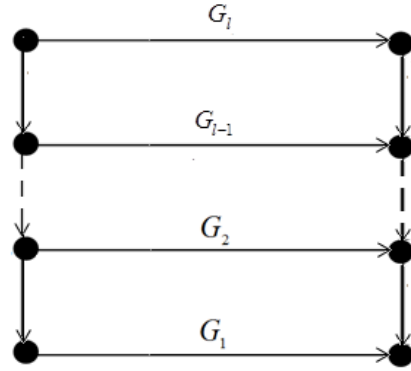
Fig. 2 The structural oriented graph \vec{G}_S^X(\tilde{V}, \tilde{U}, h)
