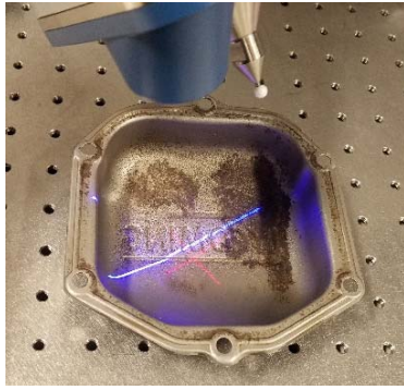
Fig. 1 Steel aircraft valve cover 3D scanning
