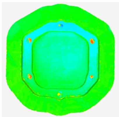
Fig. 13 3D scanning after sixth demolding process
