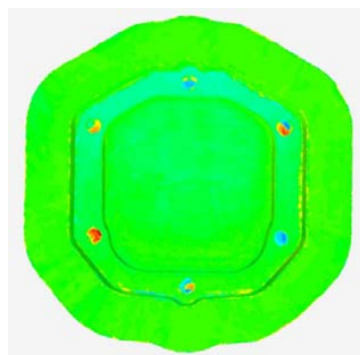
Fig. 12 3D scanning after first demolding process
