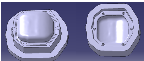
Fig. 3 CATIA designed compression mold
