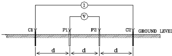
Fig. 3 Wenner four-pin Method Set-up
