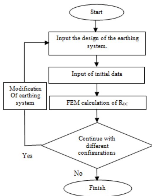
Fig. 4 Flowchart of the FEM simulation
