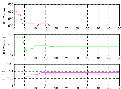
Fig. 6 Convergence of two-layer earth structure parameters
