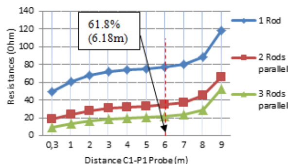
Fig. 5 Results of Earth Resistance, R_{DC}
