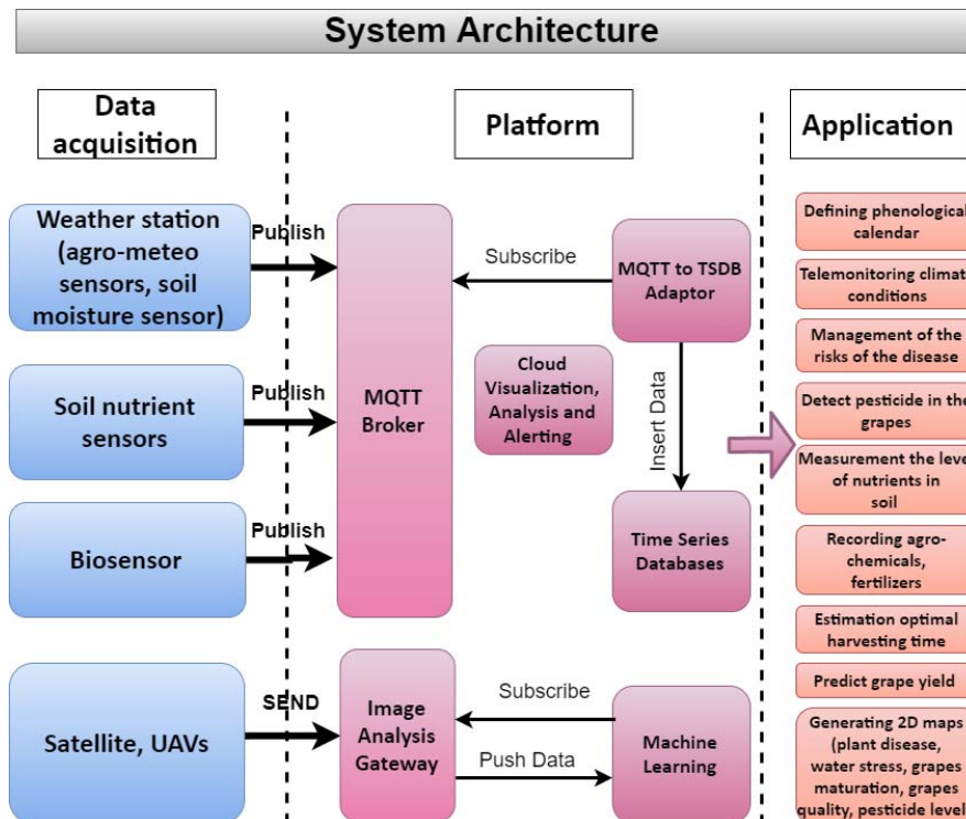
Fig. 4 DISAVIT System Architecture
