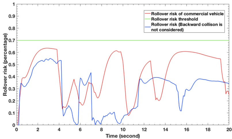
Fig. 7 (b) Rollover risk results in scenario 1
