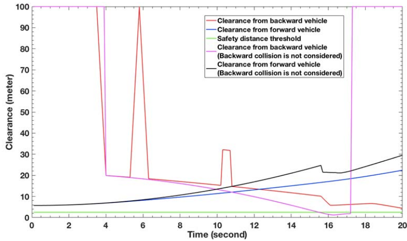
Fig. 7 (a) Clearance results in scenario 1
