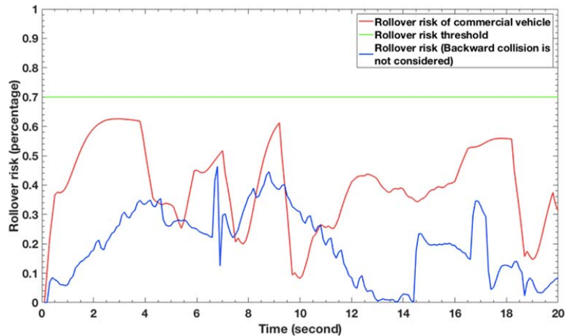
Fig. 8 (b) Rollover risk results in scenario 2
