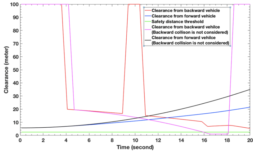
Fig. 8 (a) Clearance results in scenario 2
