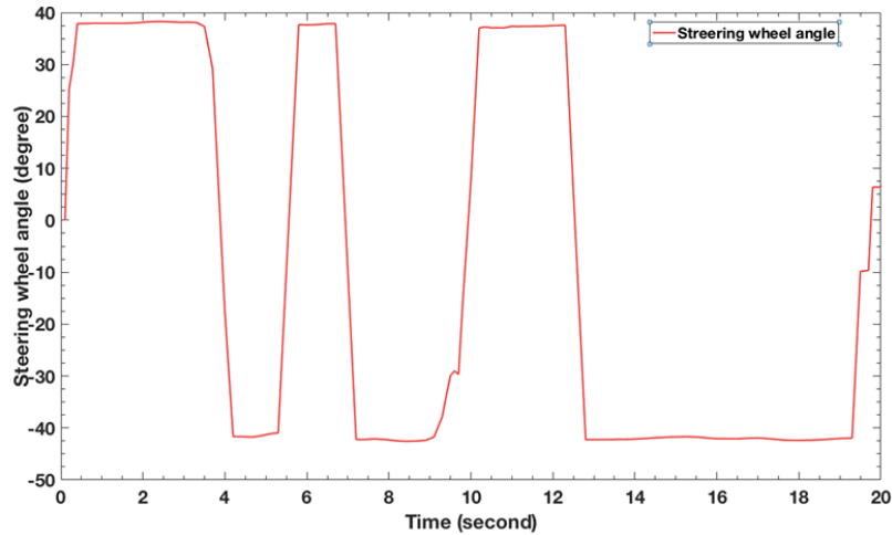
Fig. 6 (b) Control quantities of steering wheel angle
