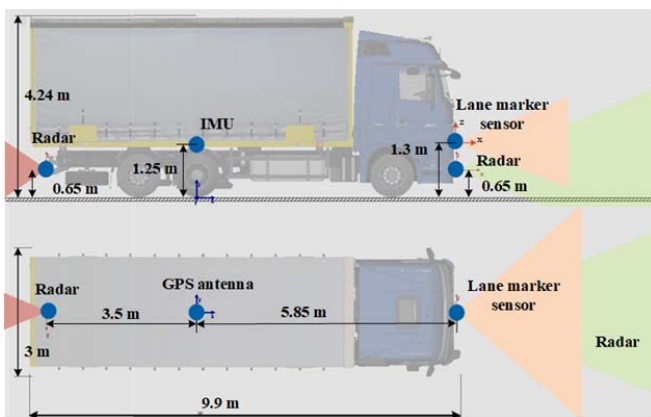
Fig. 4 Installation position of sensors on the commercial vehicle A. Training Setup
