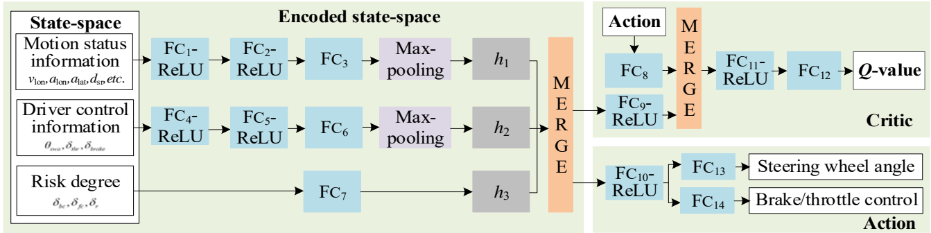
Fig. 2 Framework of the proposed actor-critic network
