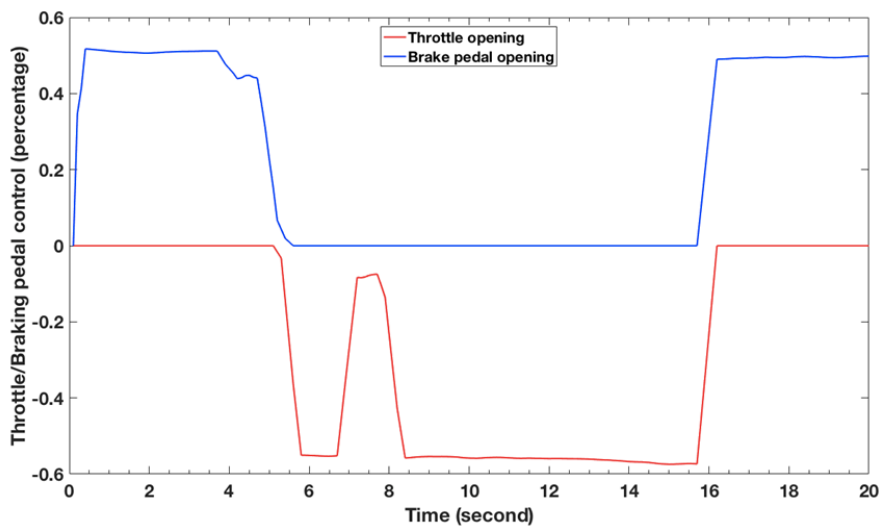
Fig. 6 (a) Control quantities of throttle/braking pedal opening
