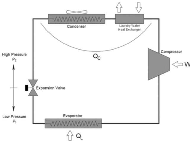
Fig. 2 Diagram of chiller cycle with heat converter
