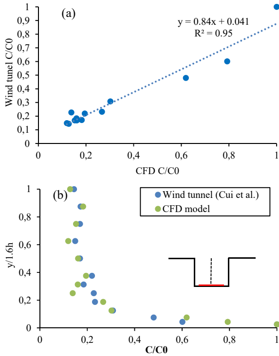
Fig. 3 CFD model of pollutant dispersal within a 2D isolated urban canyon against wind tunnel tests [22] at U_{ref}=4\text{m/s} where (a) Linear correlation between experimental and computational (b) Distribution of PM within the urban canyon
