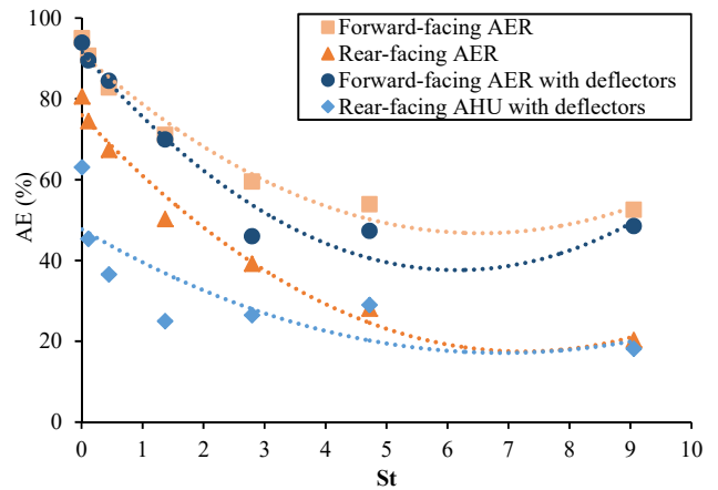
Fig. 4 AE of an AHU-AER with/without deflectors at R=1 , where the ventilation velocity is 2.5\ \text{m/s}
