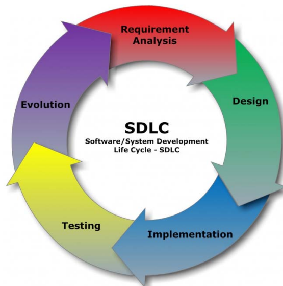
Fig. 3 SDLC Cycle [9]
