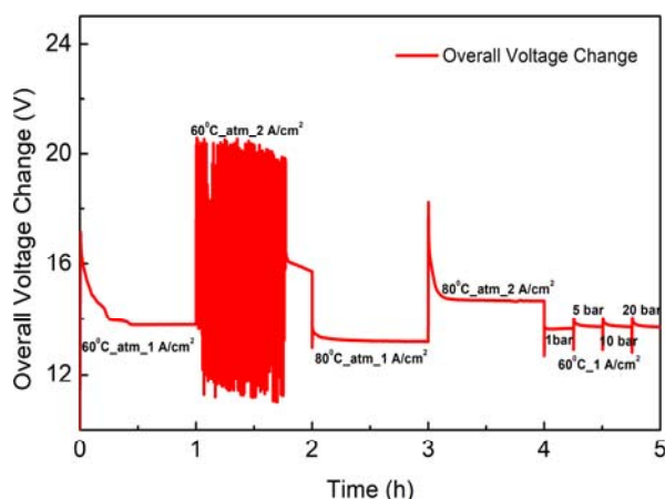
Fig. 2 The voltage change during the test period
