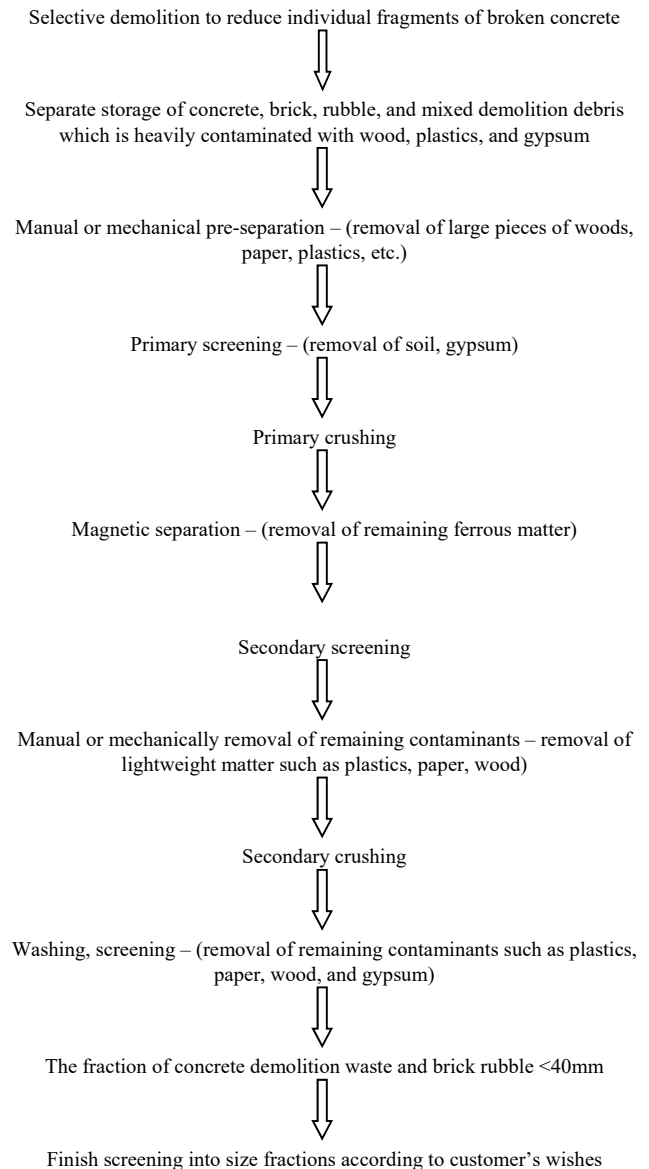
Fig. 2 Processes of construction waste materials
