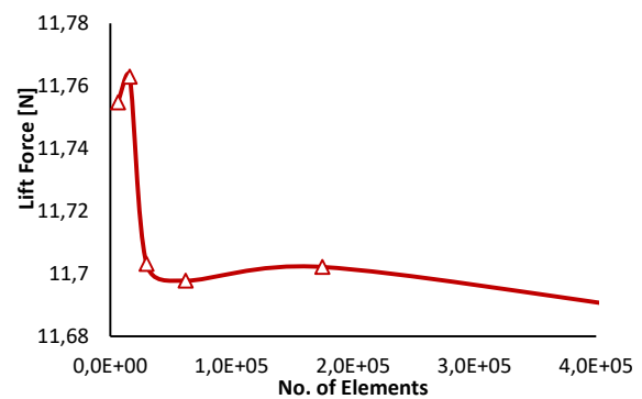
Fig. 4 Mesh Dependency Study
