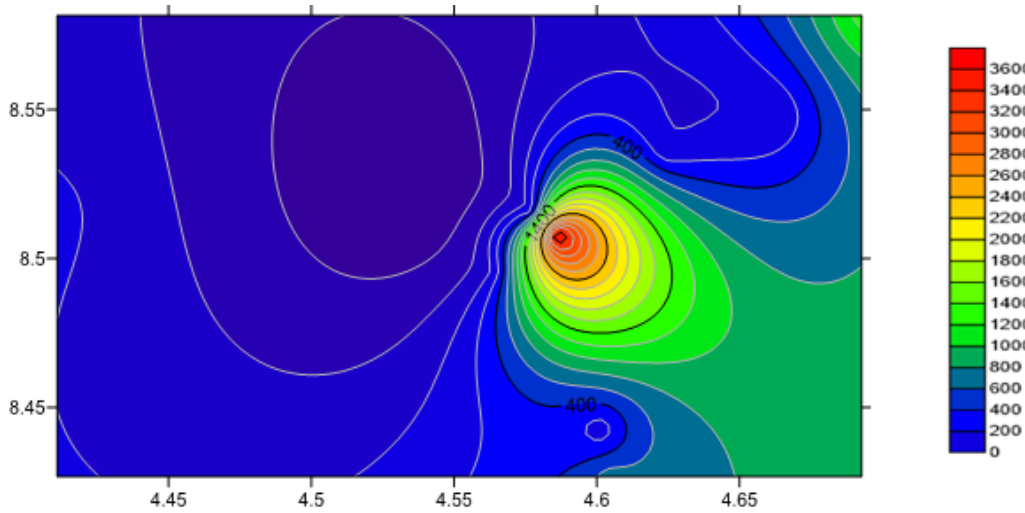
Fig. 5 (a) Isoresistivity Map of the Lateritic Layer
