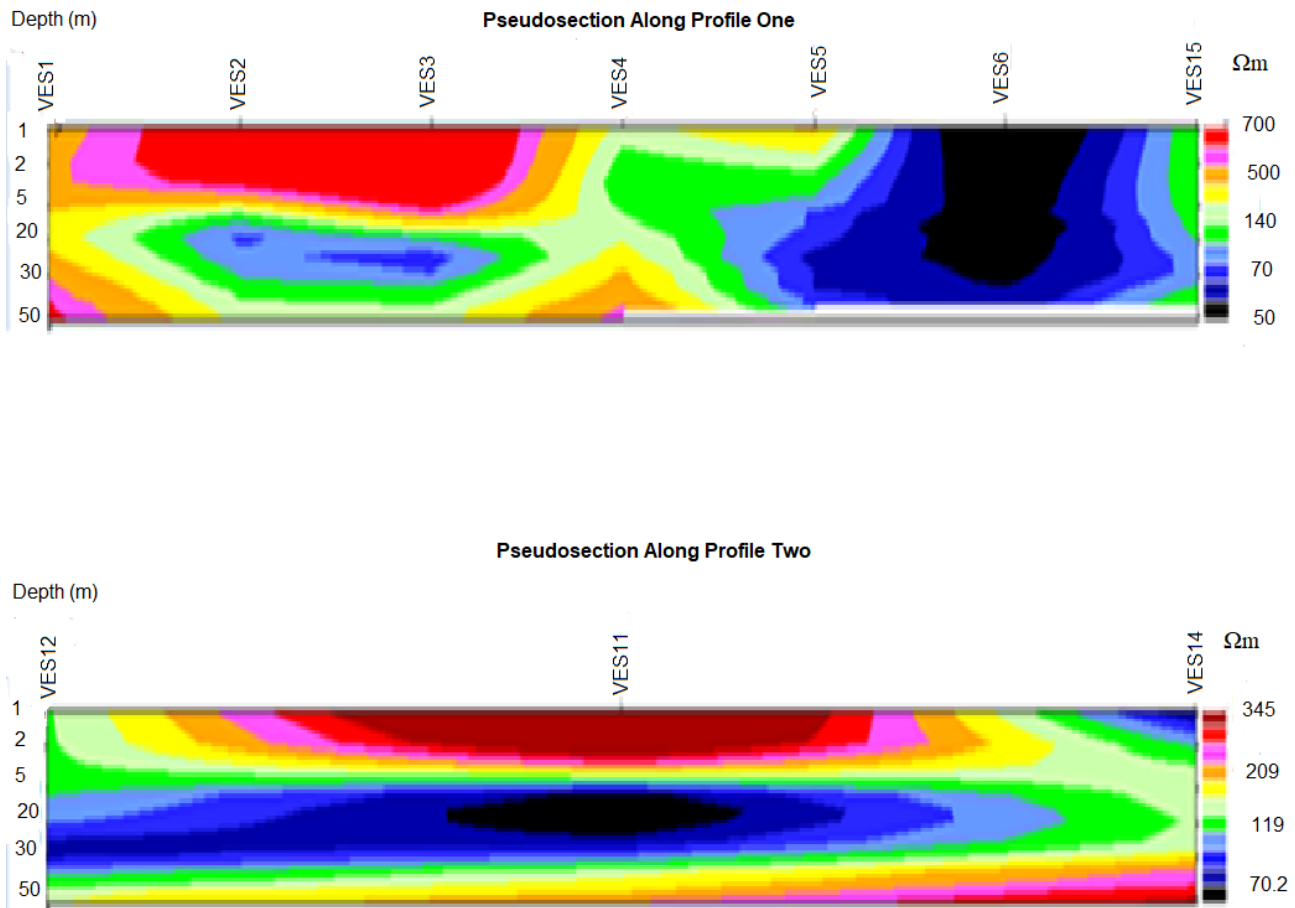
Fig. 6 Resistivity Pseudosection along Profile 1 and Profile 2
