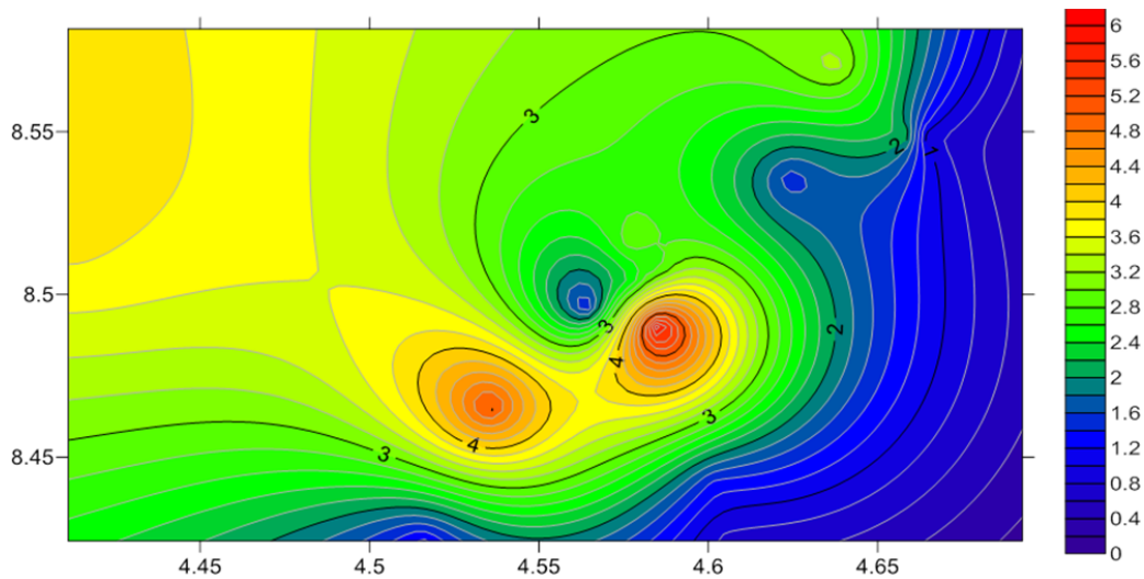
Fig. 5 (b) Isopach Map of the Lateritic Layer
