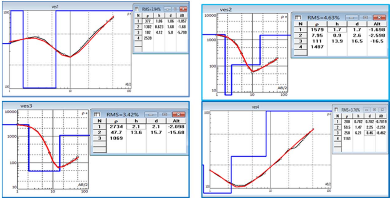
Fig. 3 Typical Sounding Curves from the Study Area
