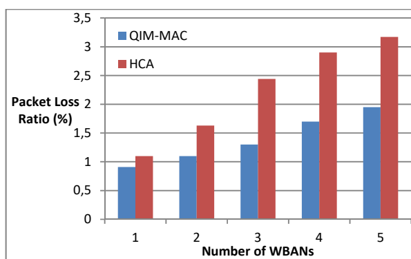
Fig. 14 Packet Loss Ratio vs Number of WBANs
