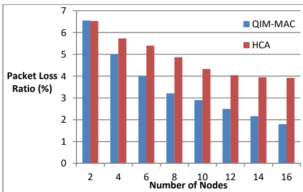
Fig. 9 Packet Loss Ratio vs Number of Nodes
