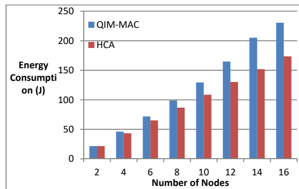
Fig. 7 Energy Consumption vs Number of Nodes
