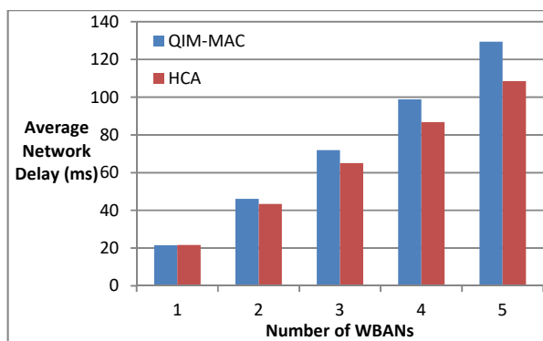
Fig. 13 Average Network Delay vs Number of WBANs
