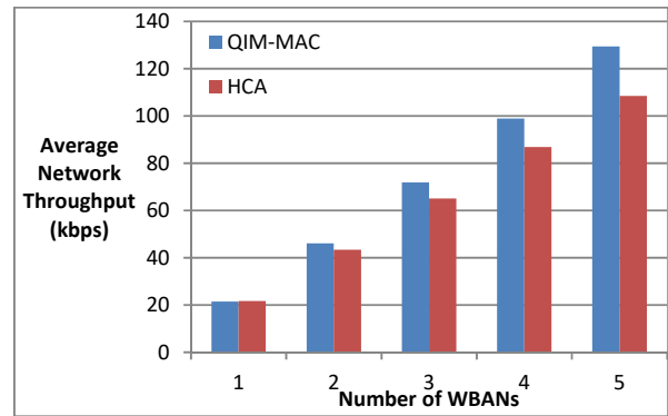
Fig. 11 Average Network Throughput vs Number of WBANs
