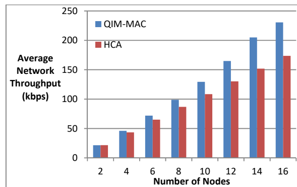
Fig. 6 Average Network Throughput vs Number of Nodes
