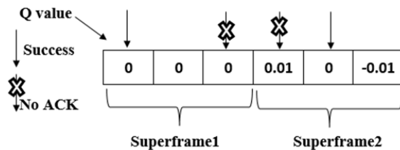
Fig. 4 Q-value for time slot on two super-frames
