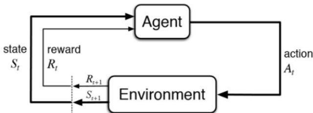
Fig. 1 Reinforcement learning
