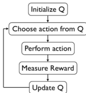
Fig. 2 Q-learning
