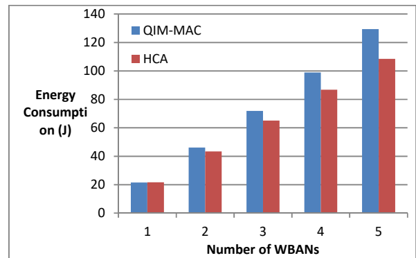
Fig. 12 Energy Consumption vs Number of WBANs
