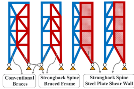
Fig. 2 Different SBS configurations
