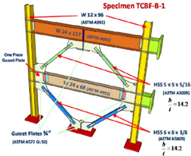
(a) TCBF-B-1 specimen configuration [14]
