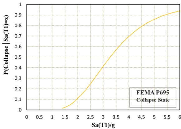
Fig. 10 Collapse fragility curve according to FEMA P695 [4]
