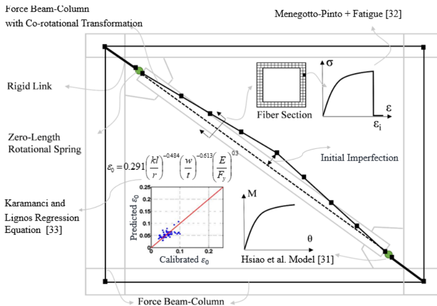
Fig. 5 Nonlinear modeling details used in this study
