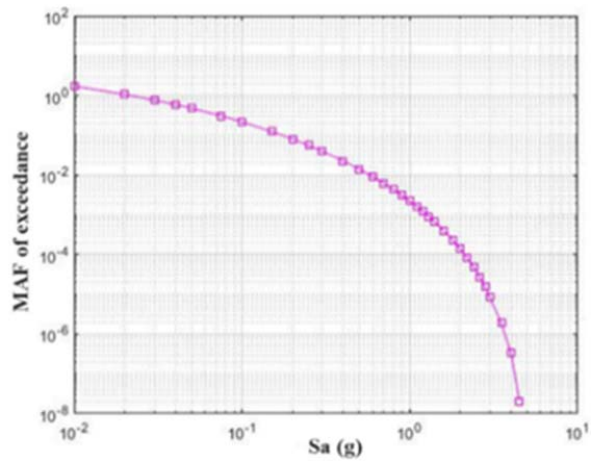
Fig. 8 Seismic hazard curve for the site
