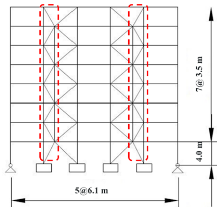
(b) Elevation of the building
