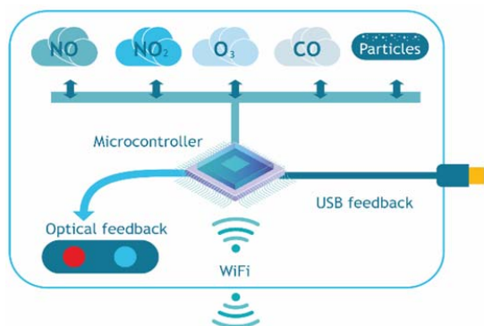
Fig. 1 Sympnia IoT platform architecture
