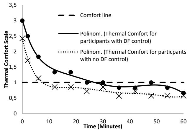
Fig. 3 Thermal comfort for occupants using CPV+DF
