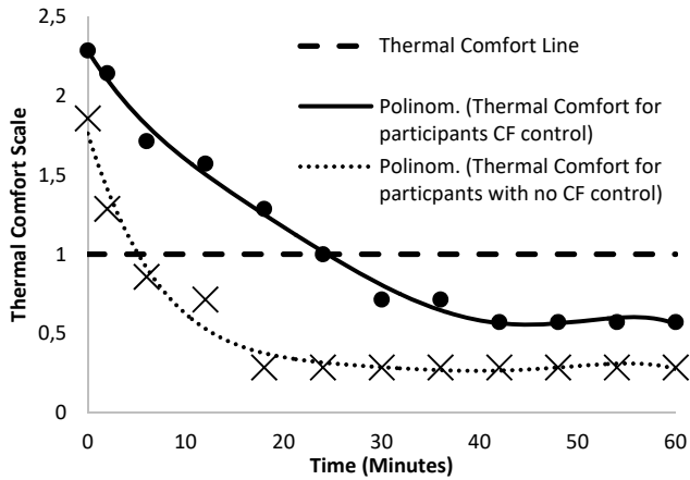
Fig. 2 Thermal comfort for occupants using CPV+CF
