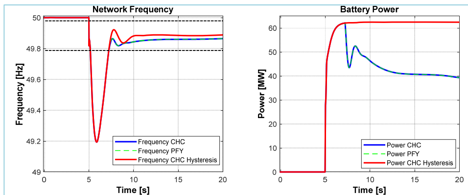
Fig. 9 Small deadband (deadband = 10 mHz and d_{fmax} = 210 \text{ mHz} ) configuration with frequency deviation reduced below than d_{fmax}
