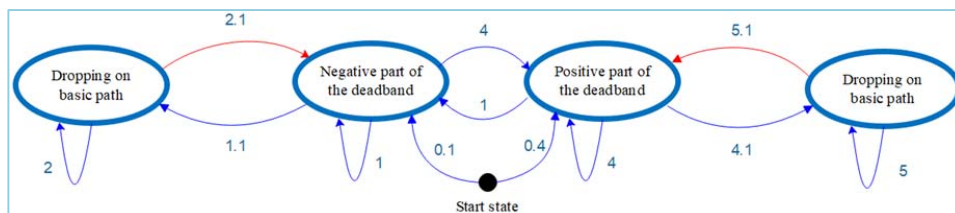
Fig. 6 State Transition Diagram (Basic BESS principle)
