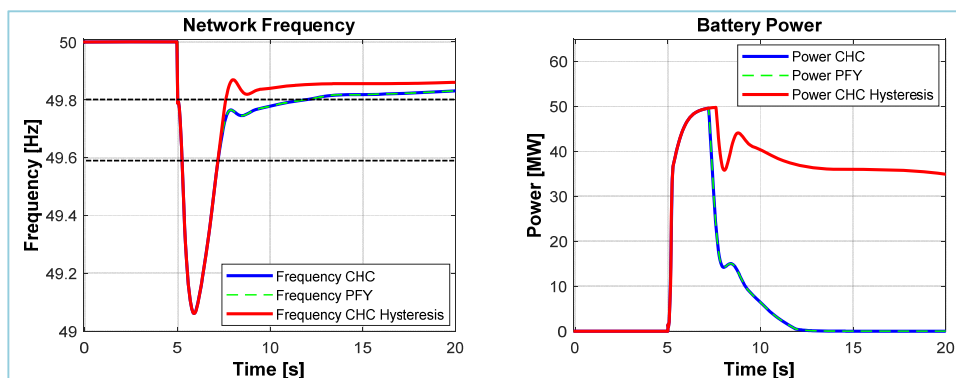
Fig. 10 Large deadband (deadband = 200 mHz and d_{fmax} = 400 \text{ mHz} ) configuration at the same battery power for both BESSs
