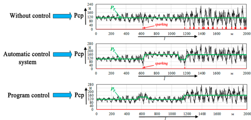
Fig. 2 Comparison of the current collector pressure control systems
