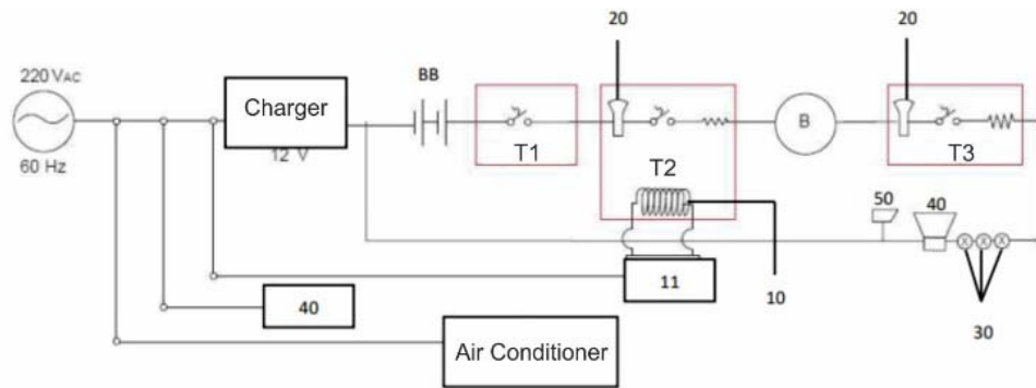
Fig. 6 Schematic electrical diagram of the device
