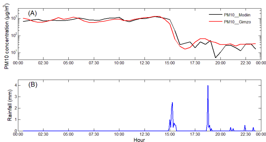
Fig. 3 Environmental measurements: (A) Measurements of PM10 pollution as taken by Modiin (black curve) and Gimzo (red curve) stations on the 9th of March 2009 between the hours of 00:30 and 23:30 of that day. The curves presented are based on half-hour averages. A sharp decline in the concentration of particulate matter as a result of rain washing is observed around 15:15-15:30. (B) The amount of precipitation (mm) as measured by the rain gauge that was situated in the city of Modi'in (in the vicinity of the local air pollution station)
