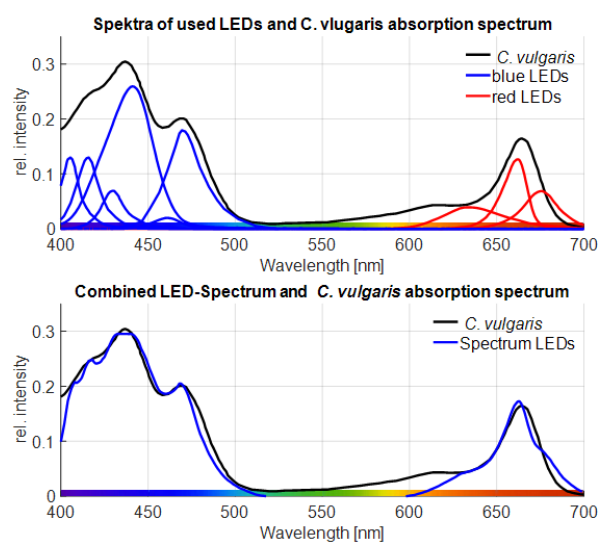
Fig. 8 Spectrum matching simulations
