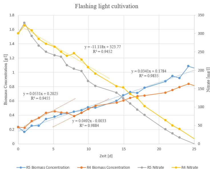
Fig. 15 OD and Nitrate concentration of Exp. 3 Run 2
