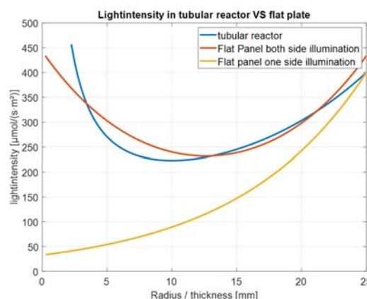
Fig. 4 Simulation of light intensity through different reactor types
