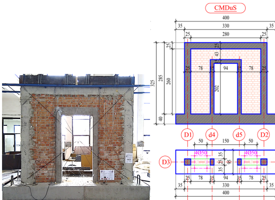
Fig. 1 Geometrical characteristics of specimens CMDuS
