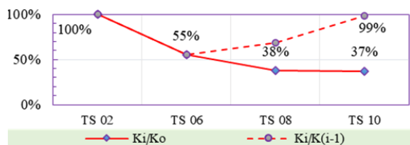
Fig. 10 Stiffness – CMDS
