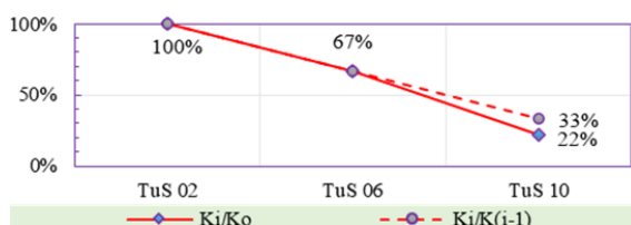
Fig. 7 Stiffness – CMDuS
