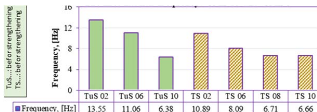
Fig. 11 The first natural frequency: CMDuS and CMDS
