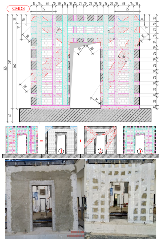
Fig. 2 Specimen CMDS
