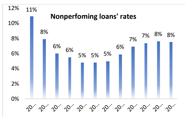
Fig. 2 The evolution of nonperforming loans' rates
