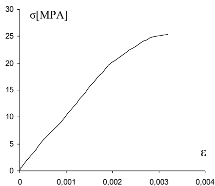
Fig. 10 Mean curve \sigma = f(\epsilon) for W = 0.6\%
