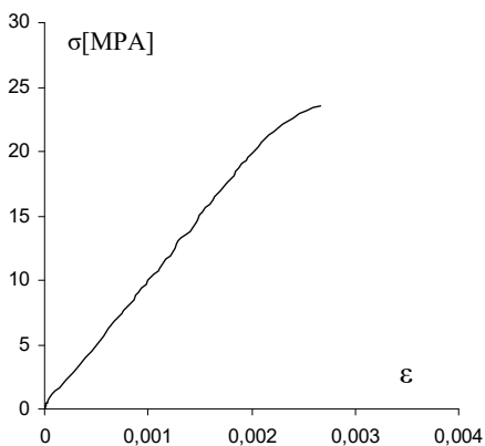
Fig. 12 Mean Curve \sigma = f(\epsilon) for BT ( W = 0\% )
