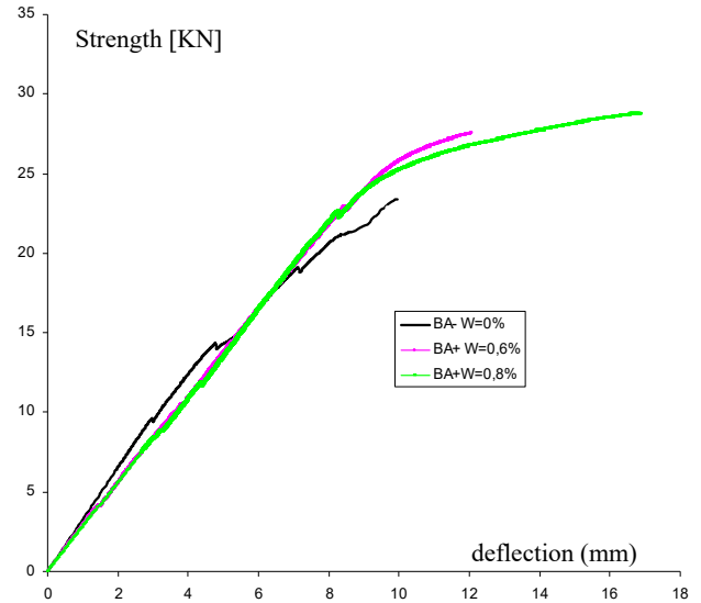
Fig. 9 Superimposition of the strength–deflection curves
