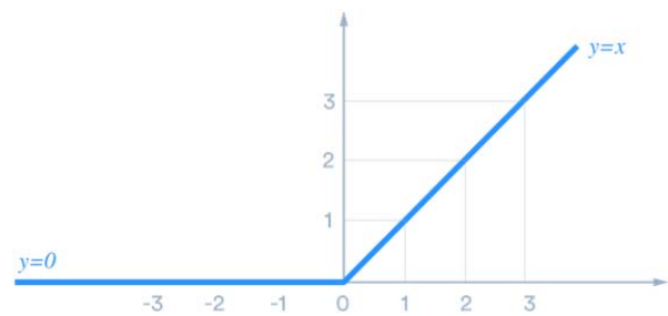
Fig. 8 ReLU Activation Function
