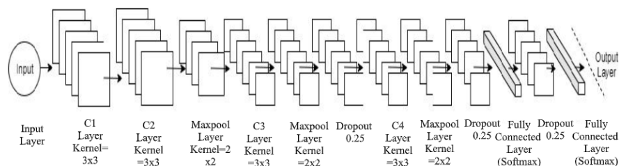
Fig. 10 Model Architecture
