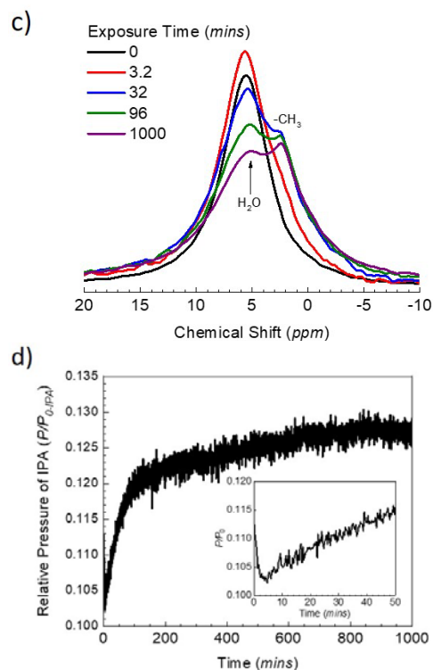
Fig. 5 (a) The IPA methyl ^1\text{H} NMR peak intensity versus time after IPA exposure of 10\ \mu\text{m} hydrophilic treated glass beads with pre-adsorbed water; (b) The water ^1\text{H} NMR peak intensity versus time after IPA exposure; (c) The ^1\text{H} NMR spectra at different times after IPA exposure; (d) The pressure tracking of competitive adsorption on 10\ \mu\text{m} hydrophilic glass beads.
