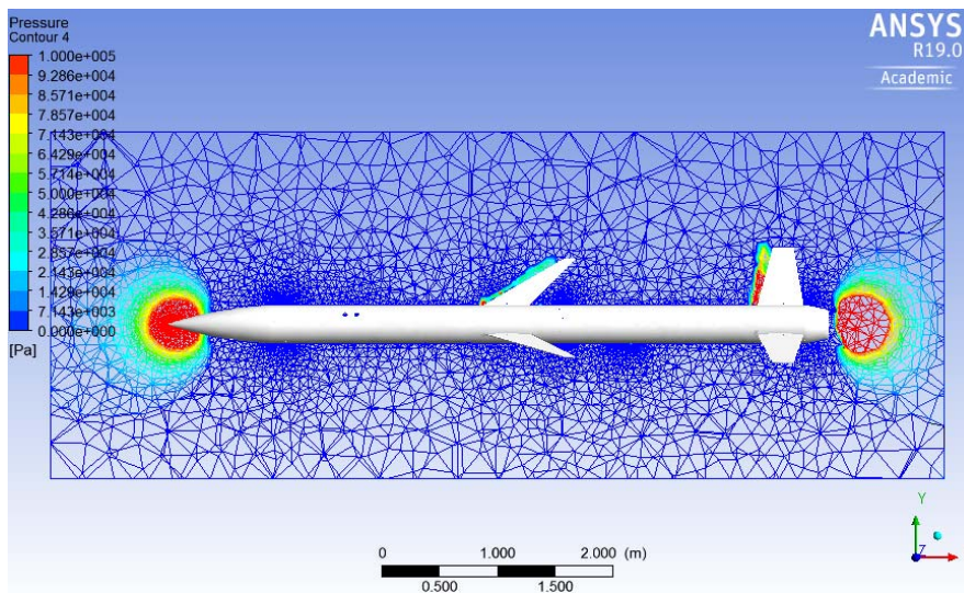
Fig. 15 Pressure contour of the rocket at Mach 6
