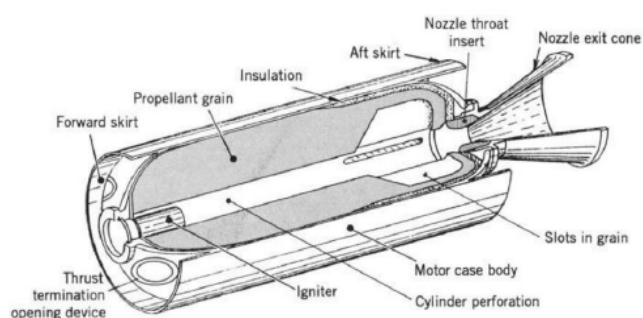
Fig. 1 Representation of a solid fuel engine [9]
