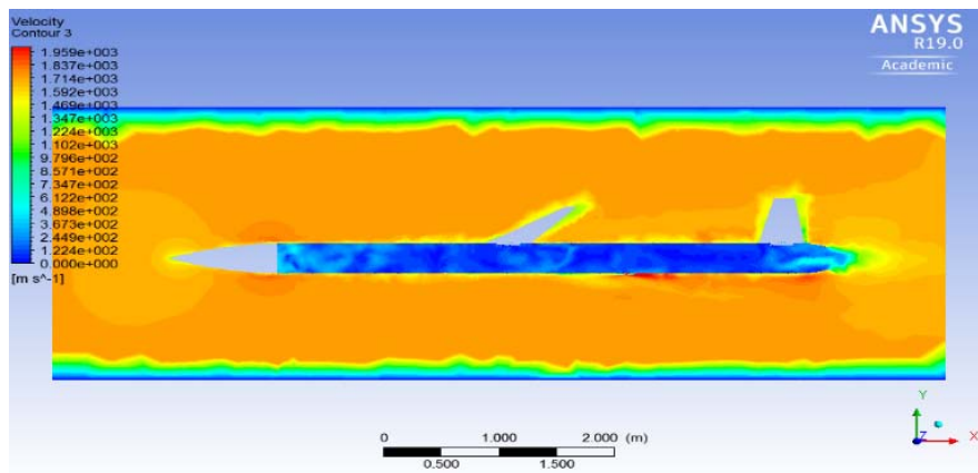
Fig. 14 Velocity contour of the rocket at Mach 6
