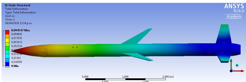
Fig. 17 Total deformation of the rocket at Mach 6
