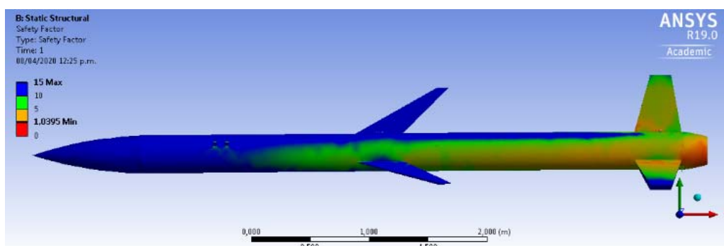
Fig. 18 Safety factor of the rocket at Mach 6
