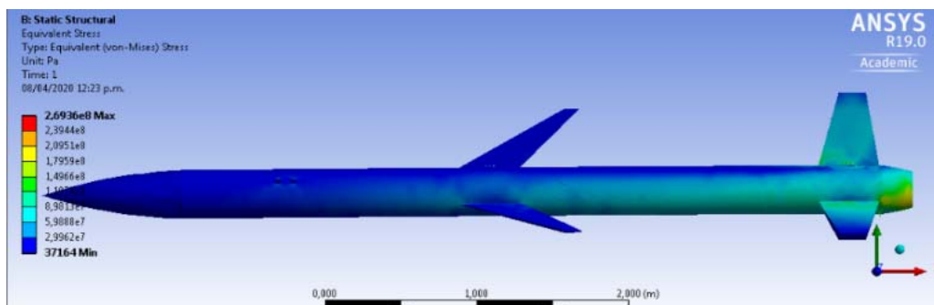
Fig. 16 Equivalent stress of the rocket at Mach 6
