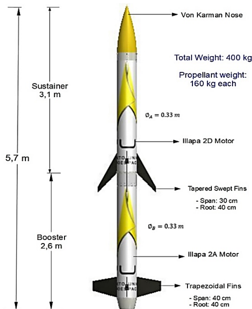
Fig. 11 Dimensions and main characteristics of the rocket
