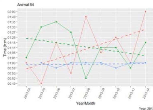
Fig. 12 Foraging state behavior duration example to Brutus (15) and Teorema (69) jaguars in 2013
