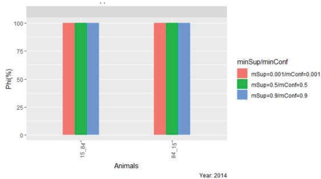
Fig. 8 Level Correlation between jaguars to 2014
