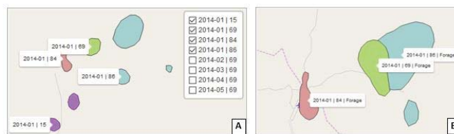
Fig. 11 (A) home range jaguar per year (B) home range jaguar per state behavior to 2014
