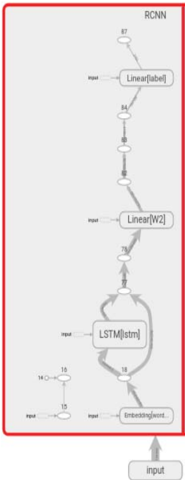
Fig. 3 RCNN architecture
