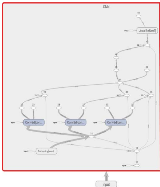
Fig. 1 CNN architecture
