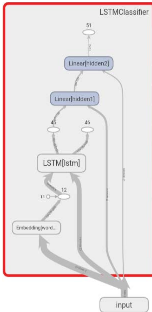
Fig. 2 LSTM architecture
