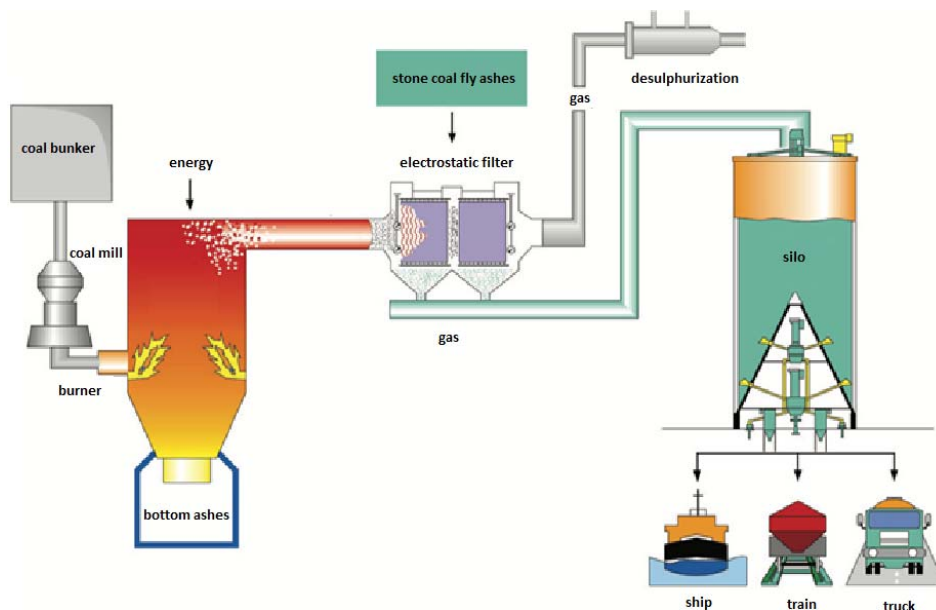
Fig. 2 Production process in the power plant [3]
