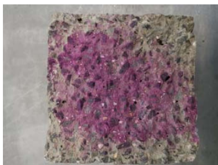
Fig. 3 Determination of the pH value on hardened concrete with the wood ashes No. 2, Table V, phenolphthalein as Indicator
