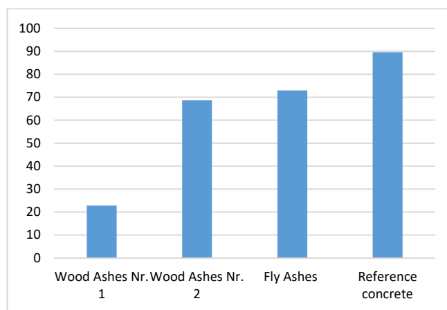
Fig. 3 Composition of compressive strength on concrete with wood and fly ashes
