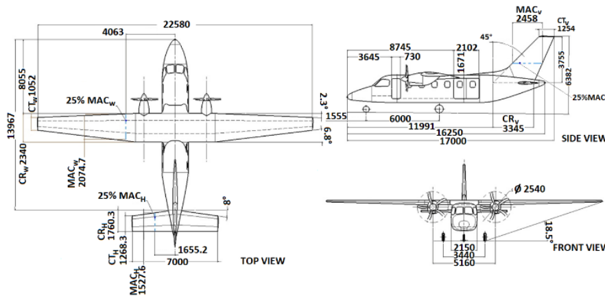
Fig. 1 Reference A/C three-view
