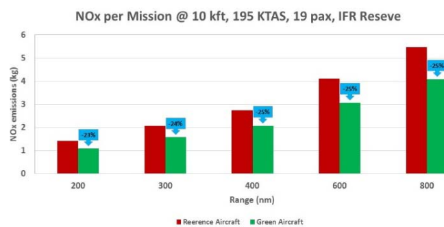
Fig. 13 NO x per mission comparison between Reference and Green A/C for the mission at 195 KTAS
