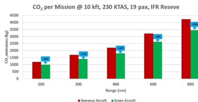
Fig. 12 CO 2 per mission comparison between Reference and Green A/C for the mission at 230 KTAS
