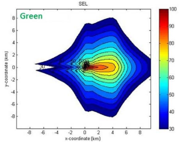
Fig. 8 SEL footprint for the Green A/C
