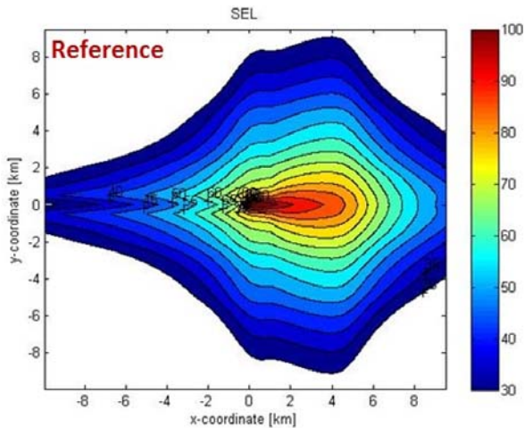
Fig. 7 SEL footprint for the Reference A/C
