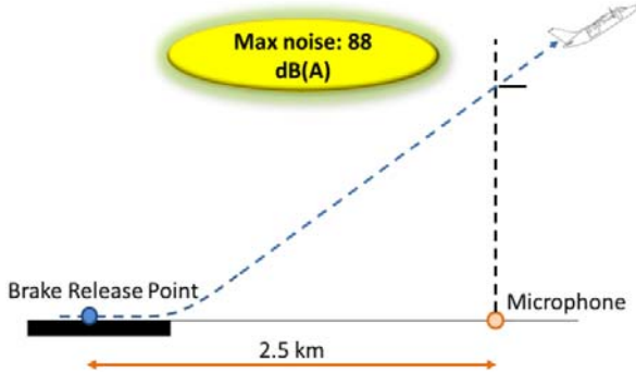
Fig. 7 Noise certification point for small commuters
