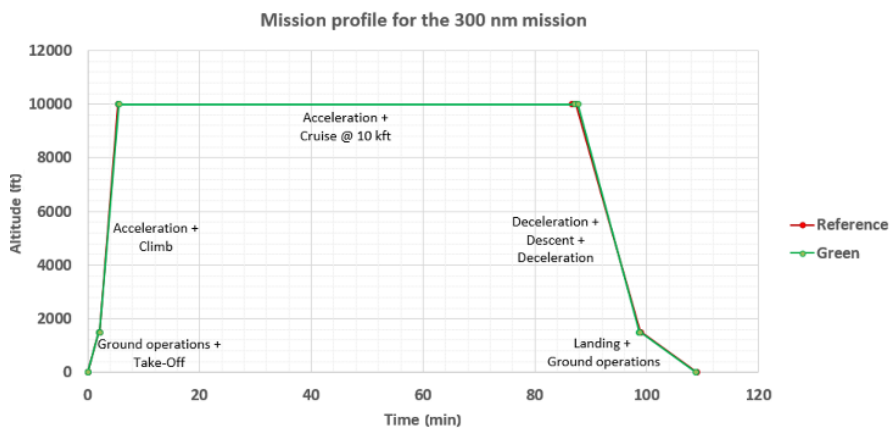
Fig. 6 Reference vs Green mission profiles
